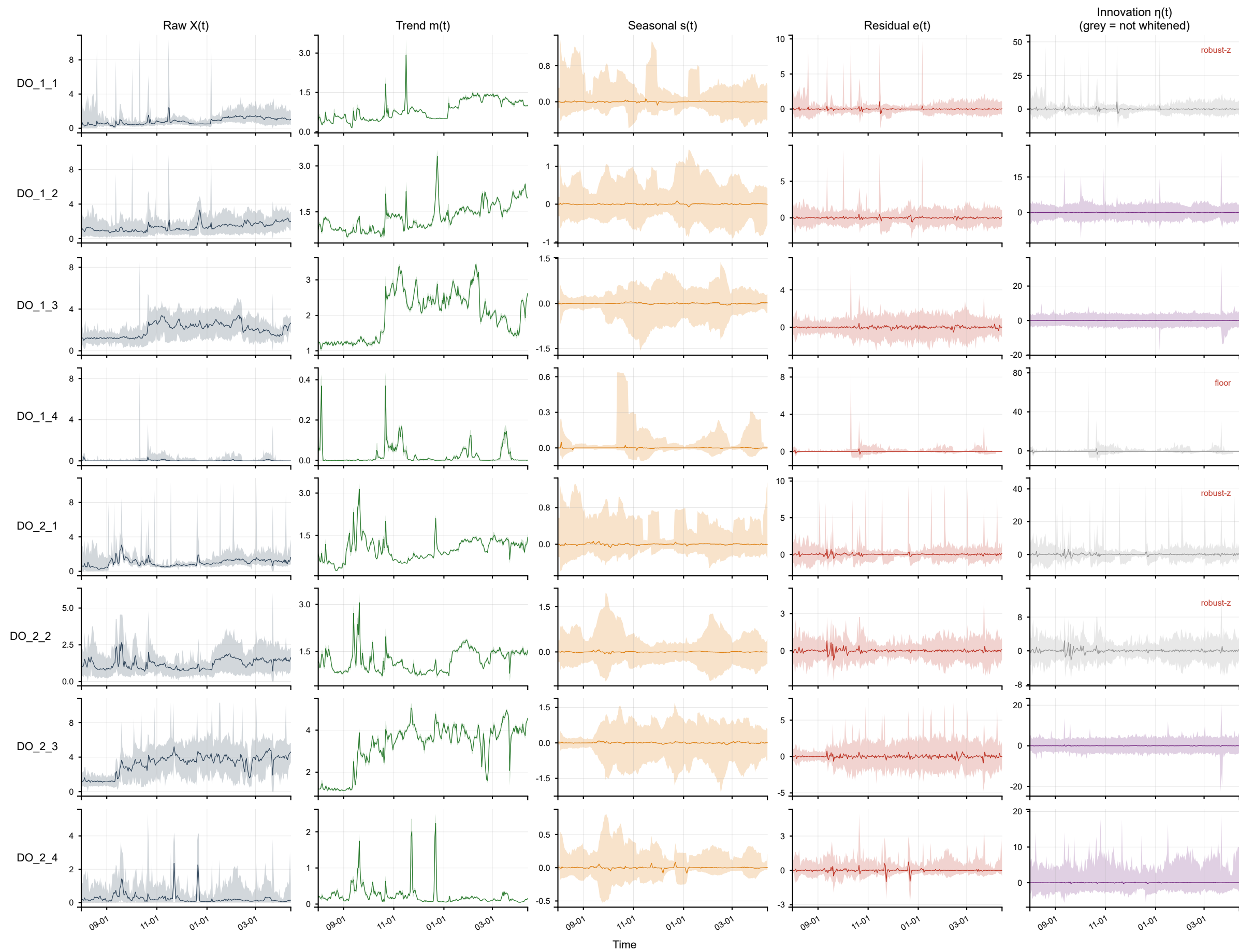
DO channels (both trains) — full-span daily overview (min–max envelope) [2025-08-01~2026-04-13]
